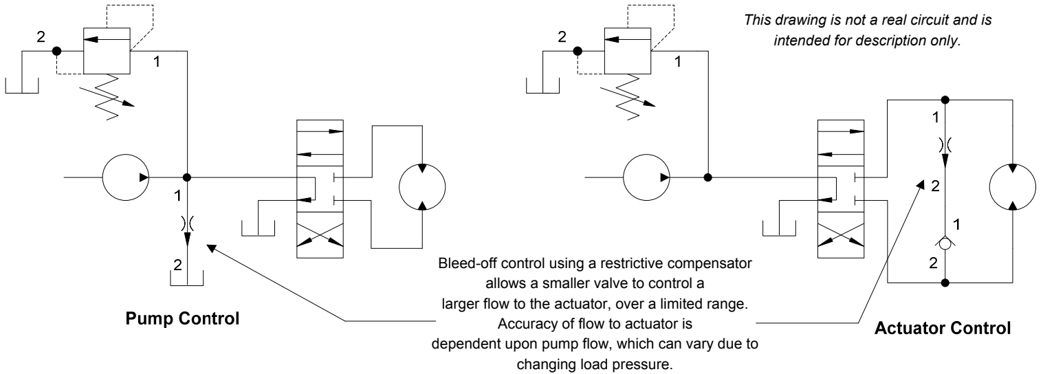
Figure 2: Bleed-Off Control for pump output flow and actuator speed
